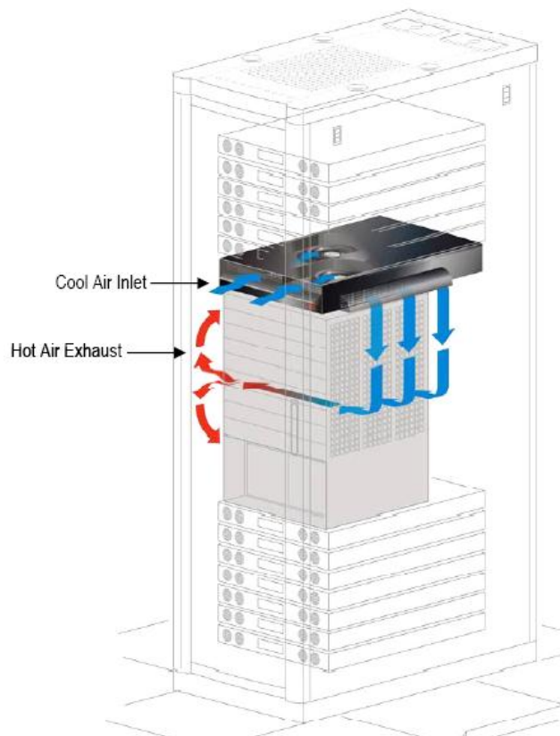
Exhibit 12: Front-view Perspective of Side-to-side Airflow with In-rack Air Distribution Equipment
