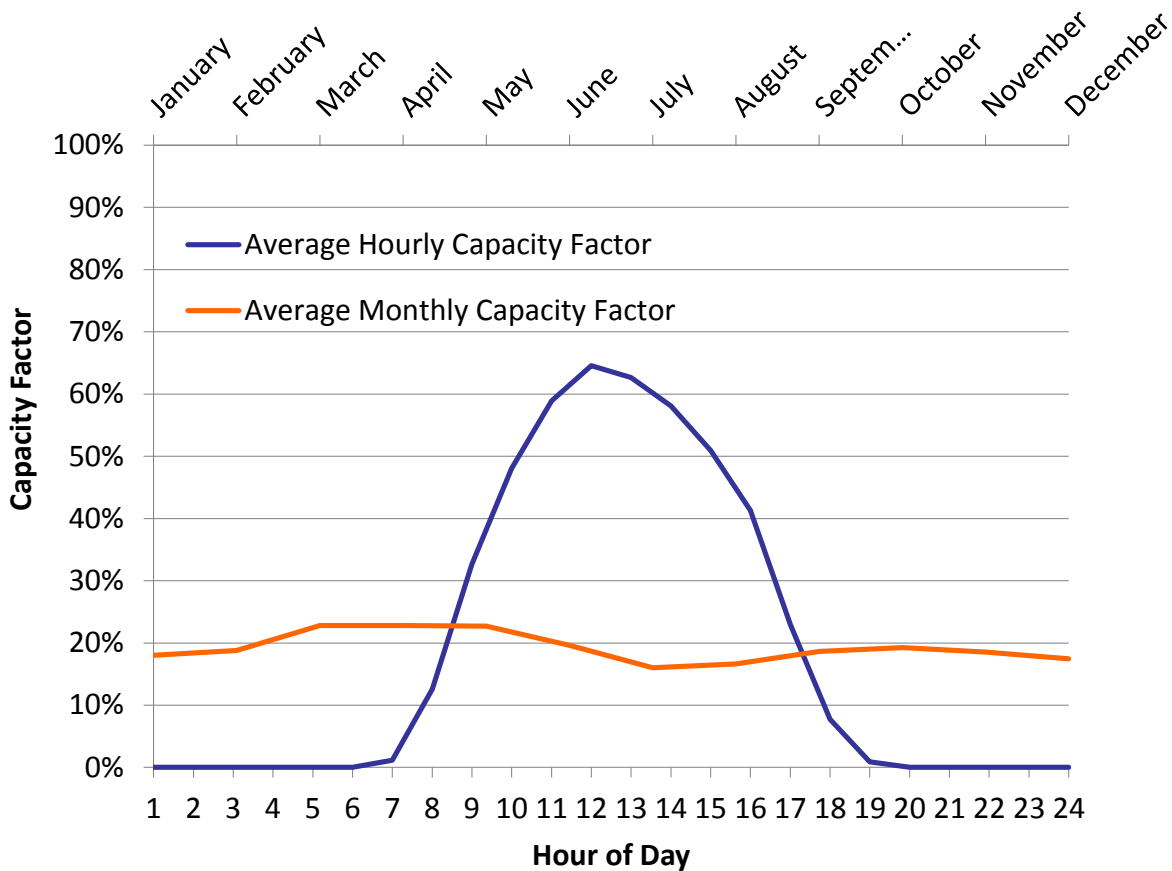
Exhibit 27: Sample Solar PV Generation Profile by Hour of Day and Month of Year
