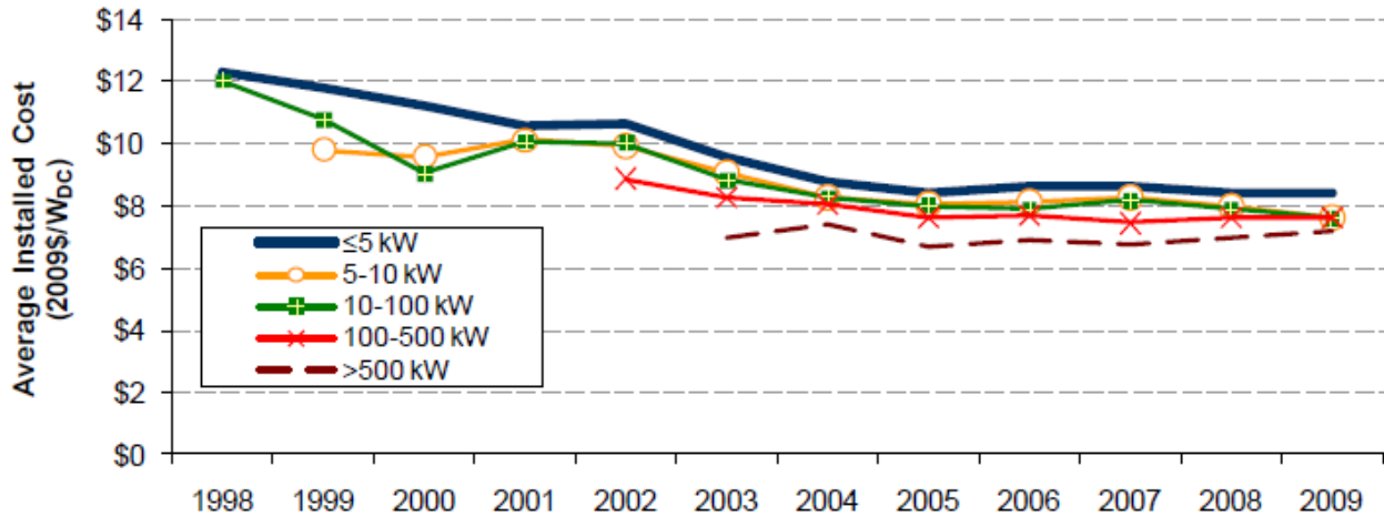
Exhibit 24: Installed Cost Trends over Time by PV System Size
