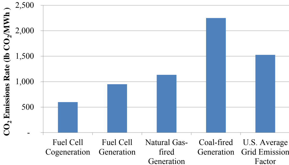
Exhibit 18: Illustrative Comparison of Power Generation and Electric Grid CO 2 Emission Rates
