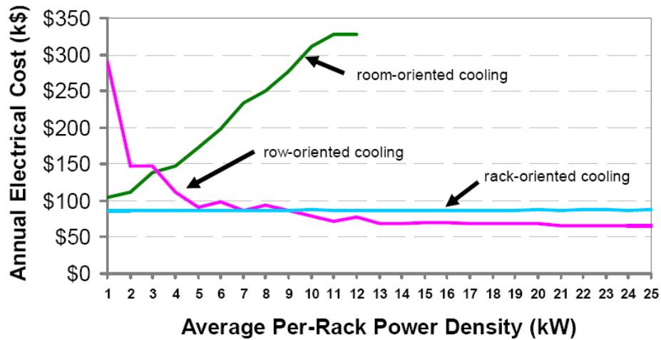
Exhibit 13: CRAC Electrical Costs as a Function of Average Rack Power Density
