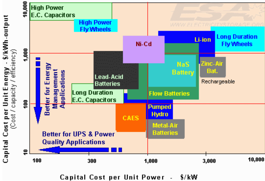
Exhibit 29: Capital Cost Estimates for Energy Storage Technologies
